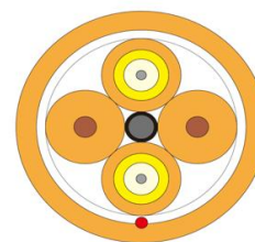
2-Core Cable with Metallic Strength Member
