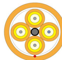
4-Core Cable with Metallic Strength Member
