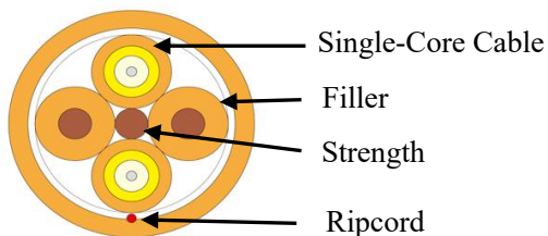
2-Core Cable with FRP Strength Member
