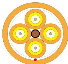
4-Core Cable with FRP Strength Member
