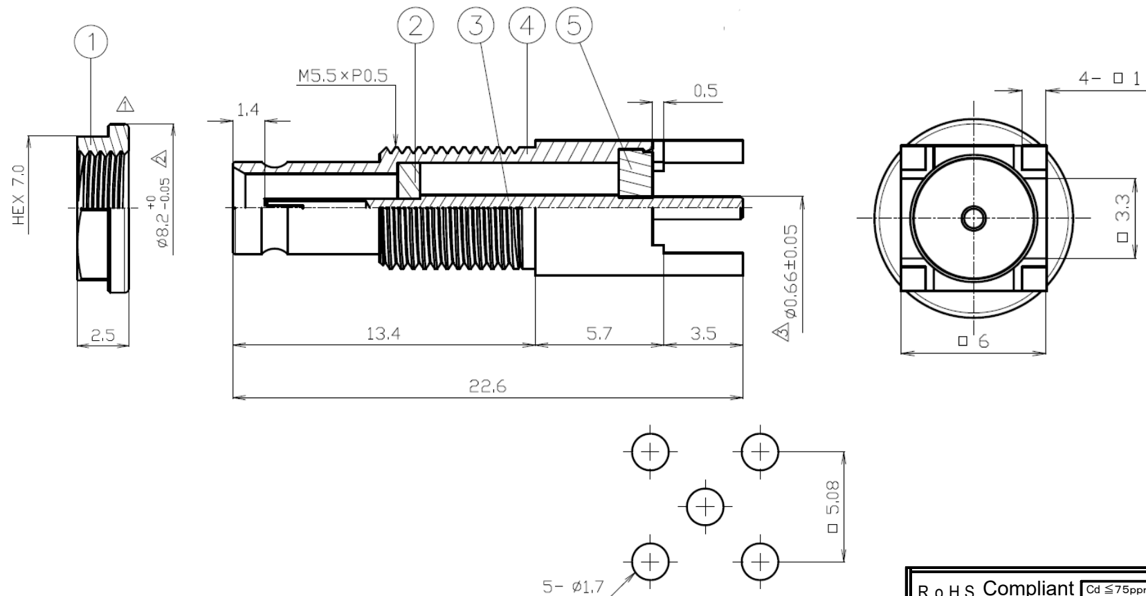
Mounting Hole Reference Dimensions
