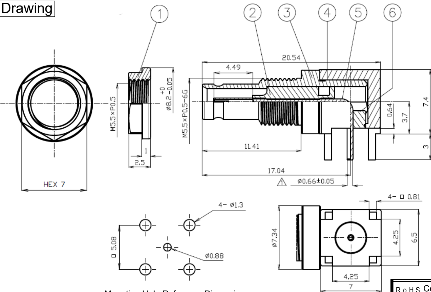
Mounting Hole Reference Dimensions
